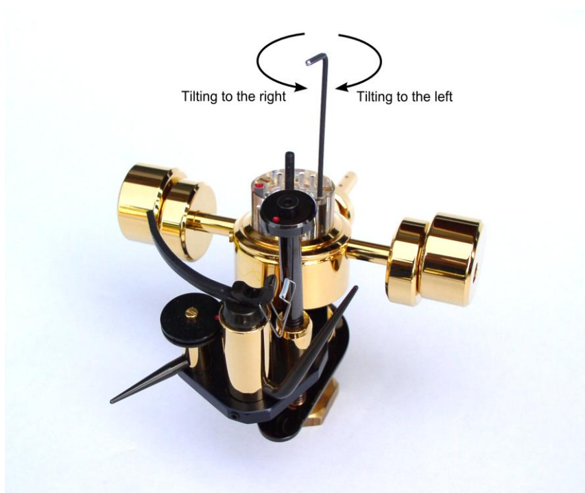
Fig. 12. Armtube is off and the hexagon key is ready to turn the pivot up or down.
