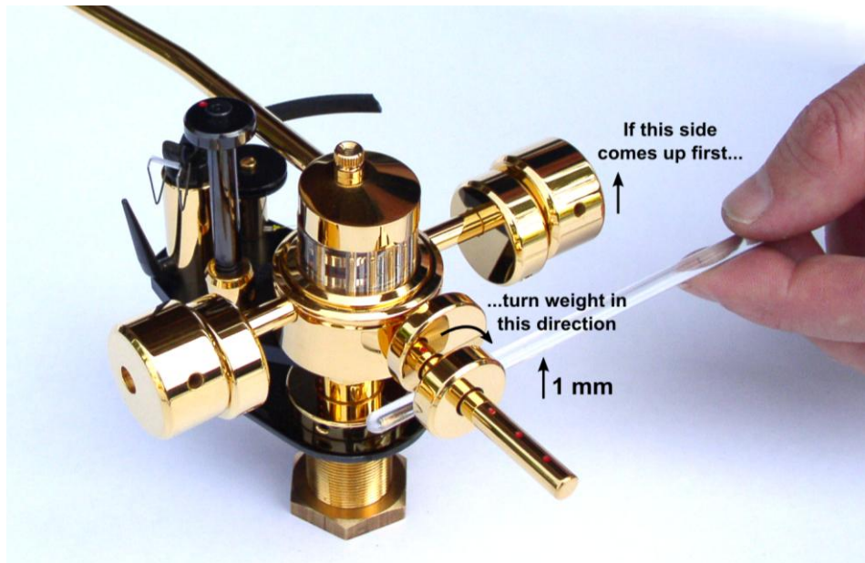
Fig. 13. Fine adjustment by turning the heavy end of any counterweight to the side that comes up first.
